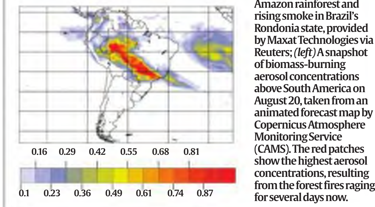
AEROSOL OPTICAL DEPTH VALUES (A measure of the extinction of the solar beam by dust and haze; the lower the value, the cleaner the atmosphere)
